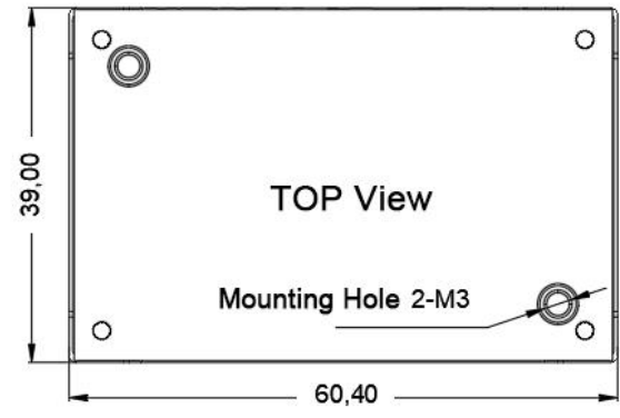
60.4*39.0*12.7mm
