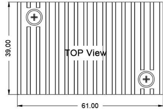
Standard+Heatsink 61.0*39.0*27.7mm
